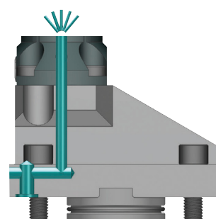
Static tool internal coolant
